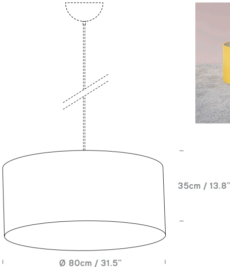
MtO: Large Drum Ø80*35: CSH8035
